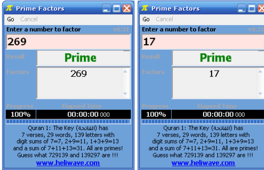
Prime Factorization of 269 and 17
