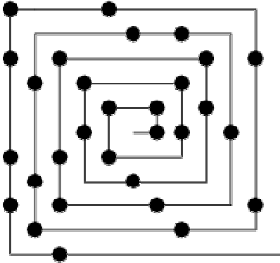
Ulam's Spiral of Prime Numbers
