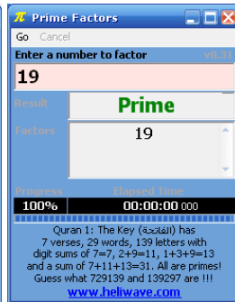
Prime Factorization of 1, 113, 5, 6229 and 19
