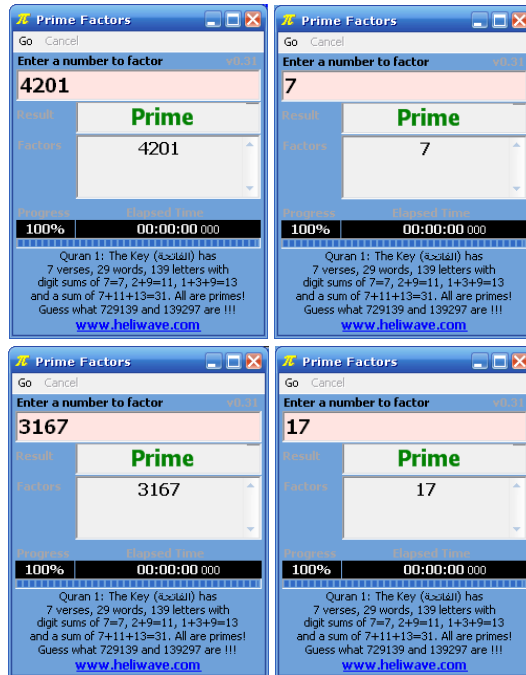
Prime Factorization of 4201, 7, 3167 and 17
