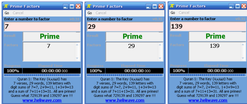
Prime Factorization of 7, 29 and 139
