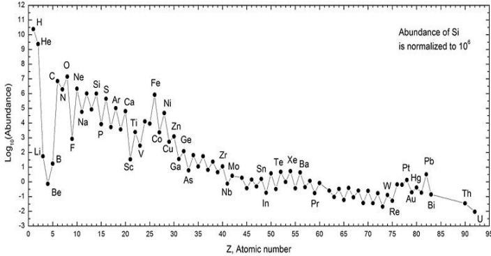
Abundance of Elements in the Solar System
