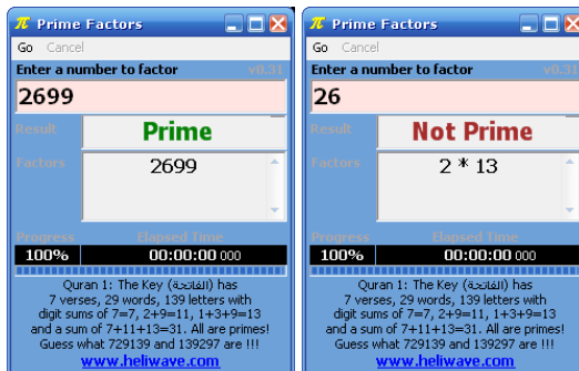
Prime Factorization of 2699 and 26
