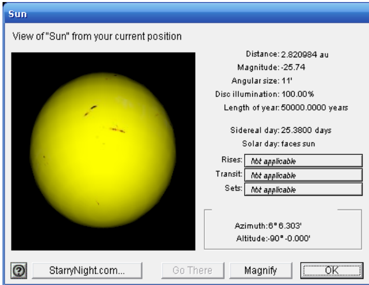
StarryNight Backyard 3.12 – Sun Info Window
